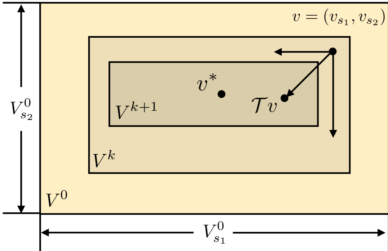
Topological interpretation of the asynchronous value iteration.
